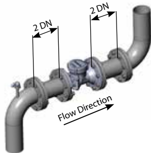
2 pipe diameters before and after elbows (90°)
